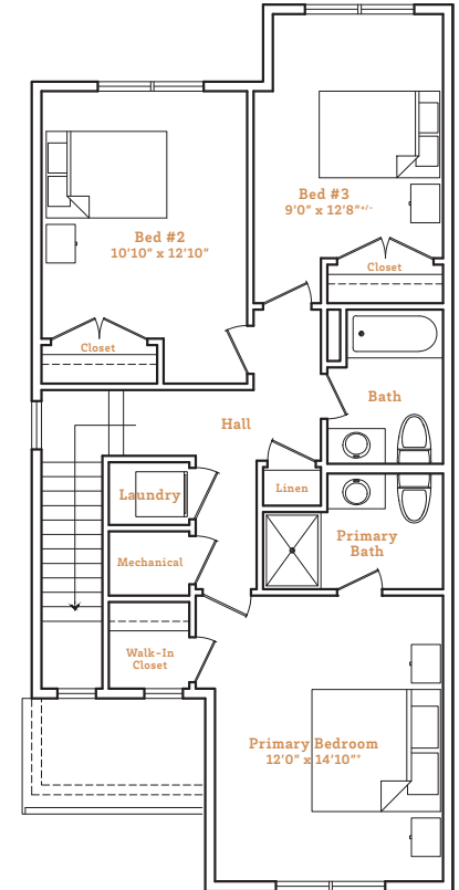
3 Bed Layout
