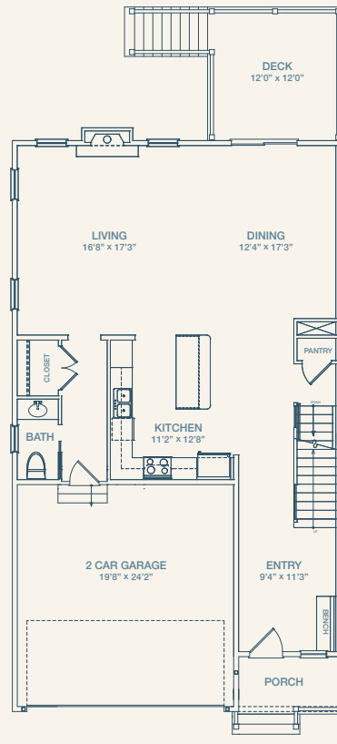
First Floor LEVEL
